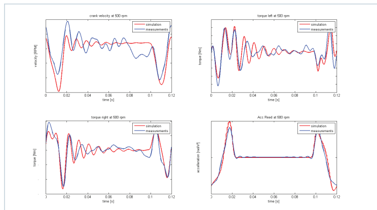
The correlation between on-site system measurements and the Simcenter Amesim/motion simulation solution from the Simcenter portfolio co-simulation model at 500 RPM.
