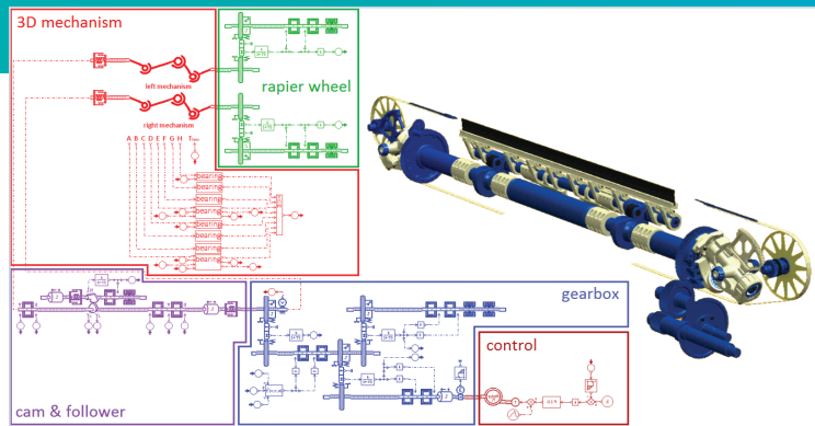
Simcenter Amesim model of the weaving machine in co-simulation with motion simulation solution from the Simcenter portfolio.
